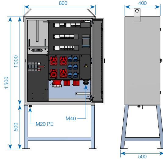
Main distributor box 100A direct measurement
